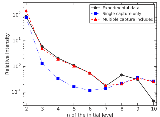
Figure 1: Experimental and calculated X-ray intensities for 1snp \rightarrow 1s^2 transitions in \text{Ar}^{16+} following electron capture in 15 \text{ keV}/q \text{ Ar}^{16+} - \text{Ar} collisions (see text for details).
